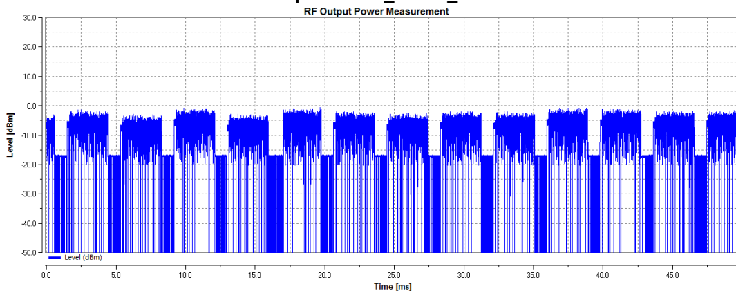
RF Output Power_TNVN_8DPSK
