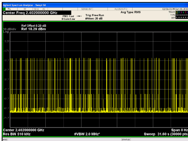
Accumulated Dwell time_TNVN_π/4DQPSK_2441
