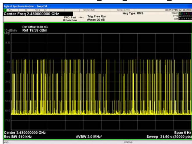
Accumulated Dwell time_TNVN_π/4DQPSK_2480
