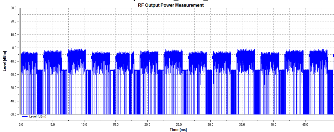
RF Output Power_THVN_8DPSK
